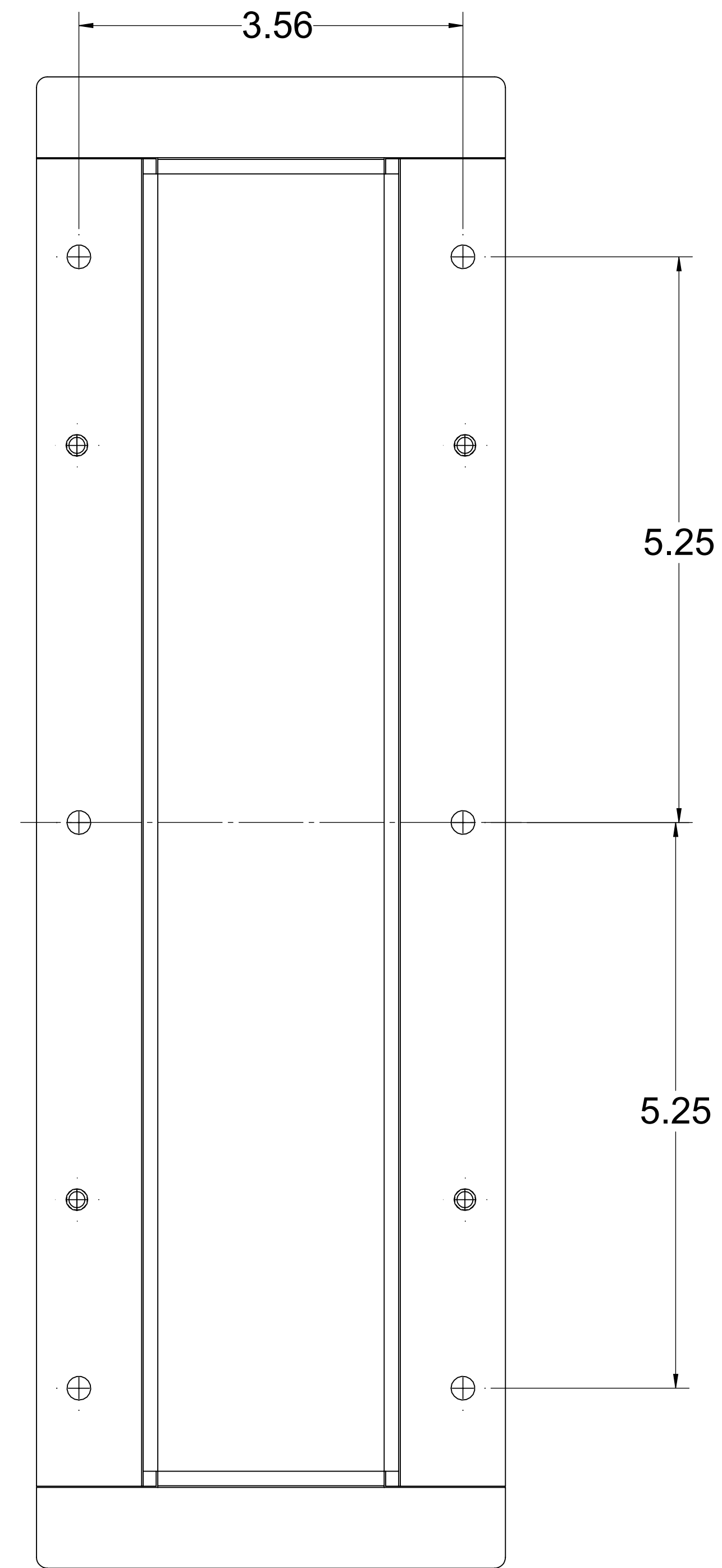
MOUNTING DIMENSIONS
