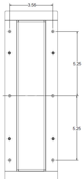
MOUNTING DIMENSIONS
