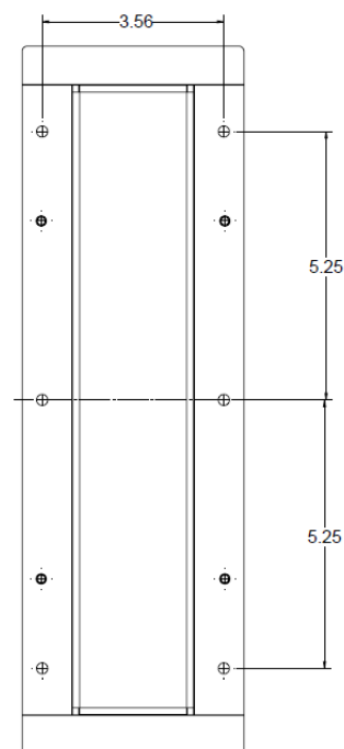
MOUNTING DIMENSIONS
